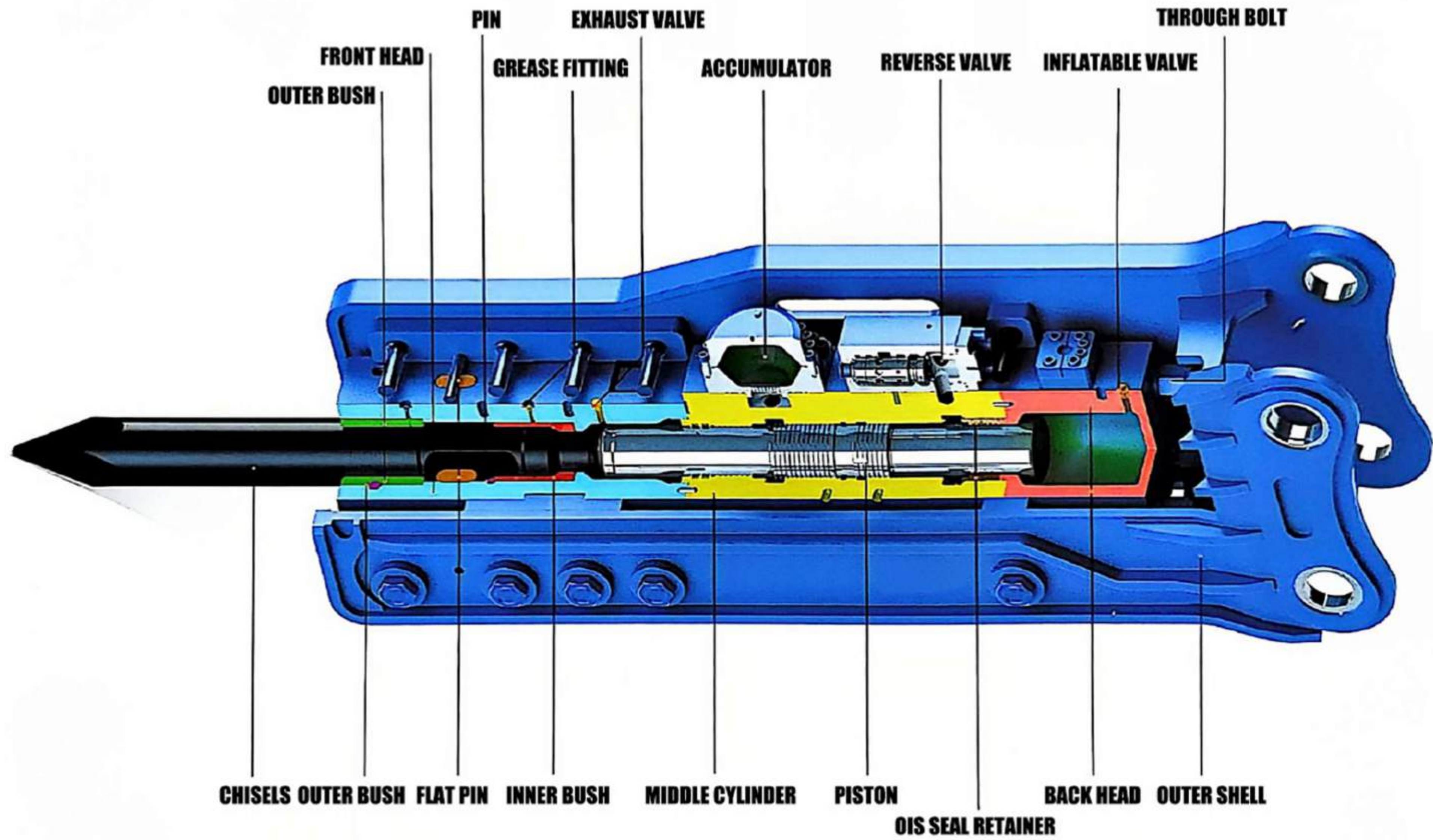
BREAKER MAIN PARTS
